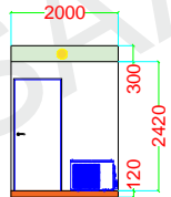
BACK SIDE ELEVATION
