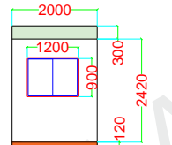
LEFT SIDE ELEVATION
